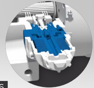
ENCAPSULATED BRAKE SYSTEM BESIDE DIFFERENTIAL
