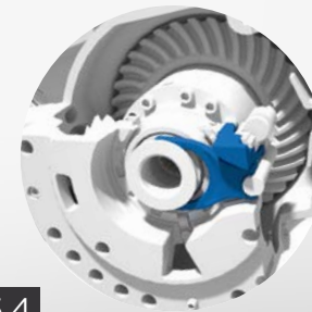
DIFFERENTIAL LOCKS DOG CLUTCH
